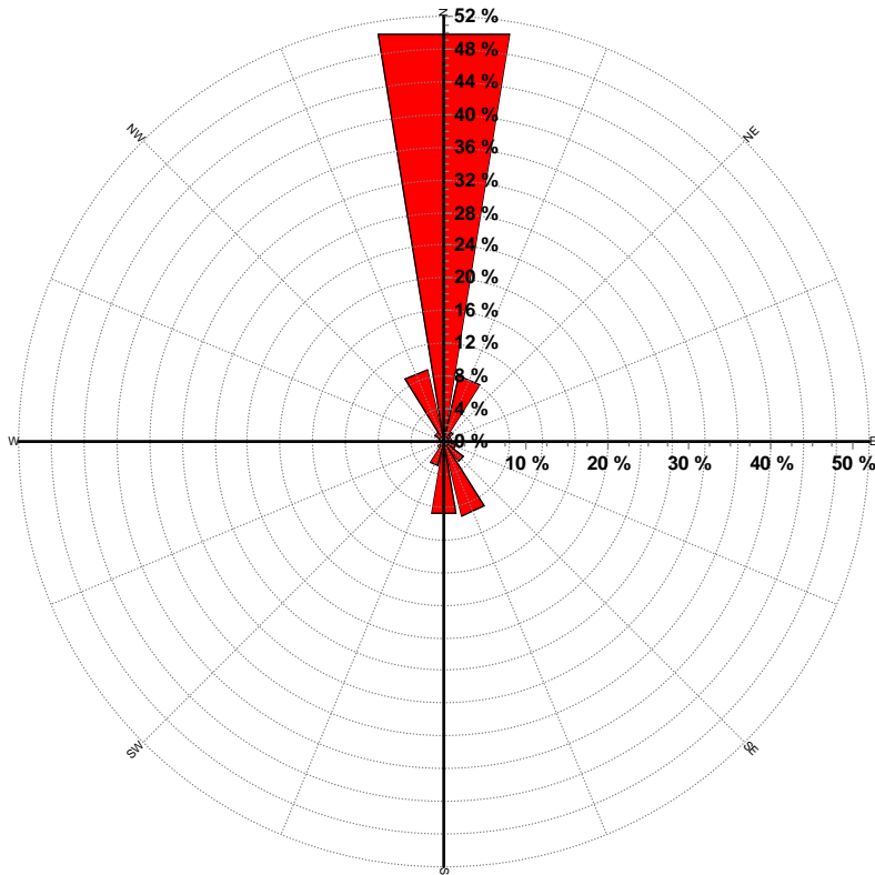
Halandras Ranch – Meeker #2 Site Wind Rose for 33 feet AGL 5/6/2003 – 9/28/2004
